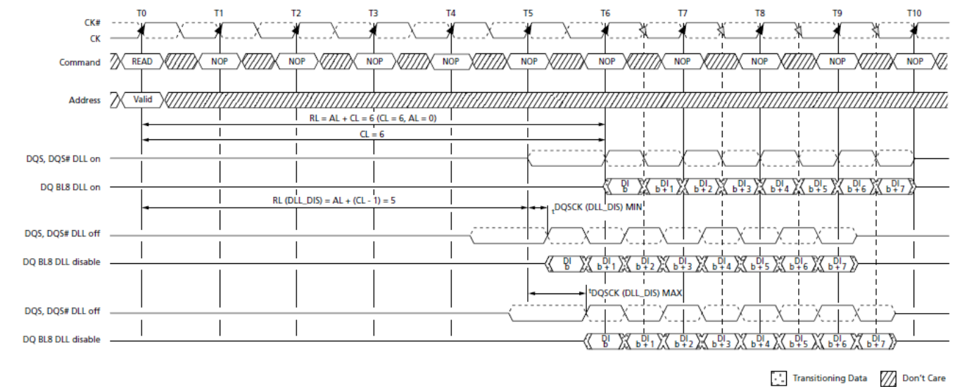
DLL Disable t_{DQSK}
