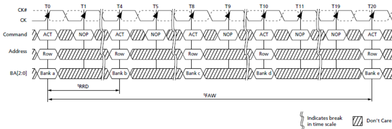
Example: t_{FAW}
