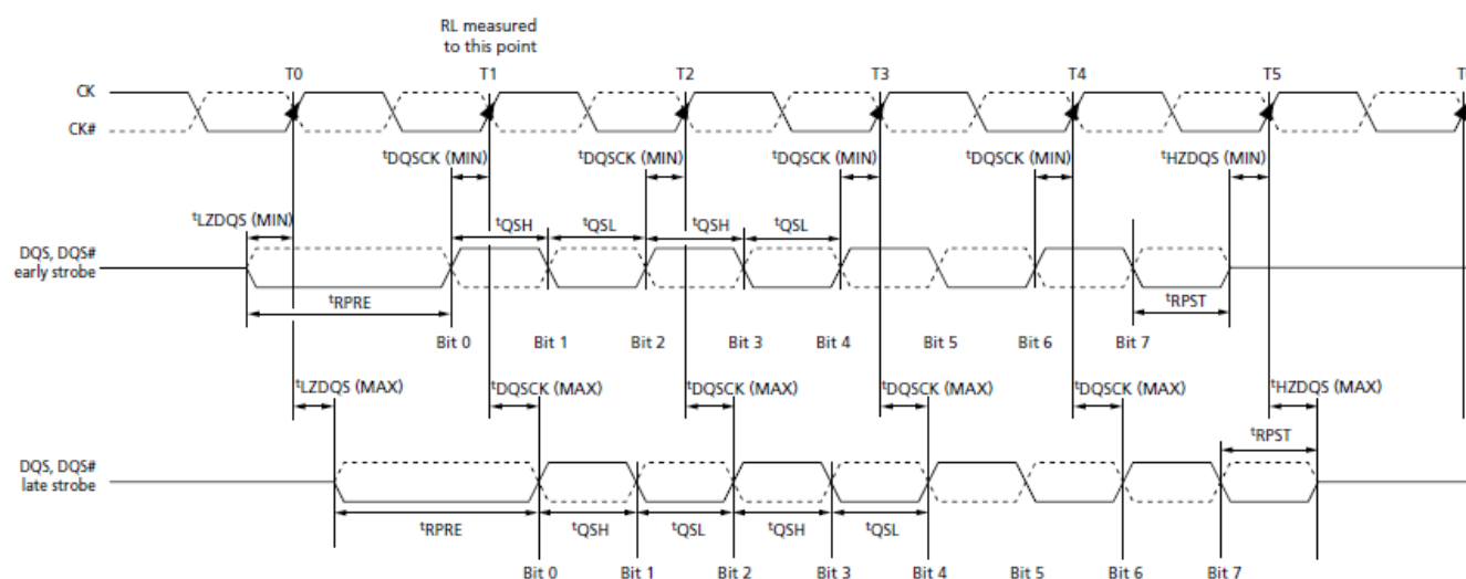
Data Strobe Timing – READs
