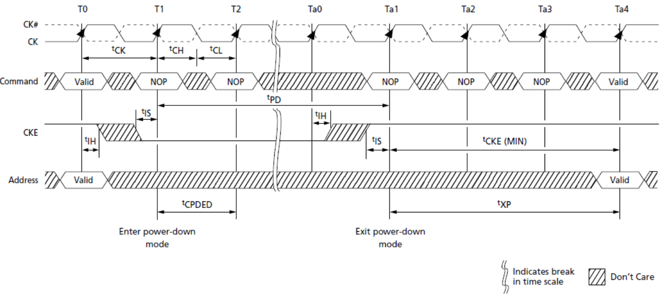
Active Power-Down Entry and Exit
