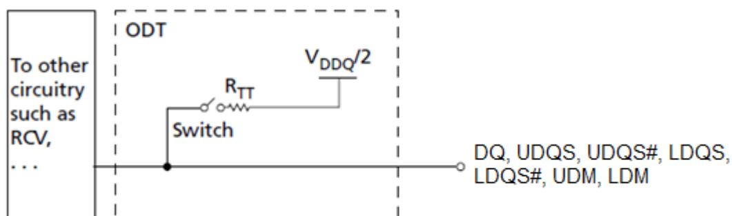
On-Die Termination
