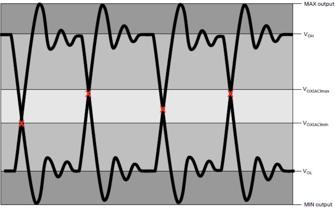
Differential Output Signal
