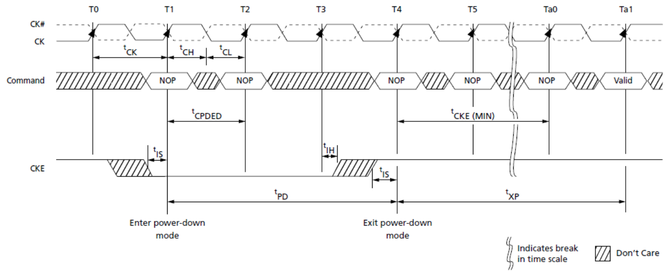
Precharge Power-Down (Fast-Exit Mode) Entry and Exit
