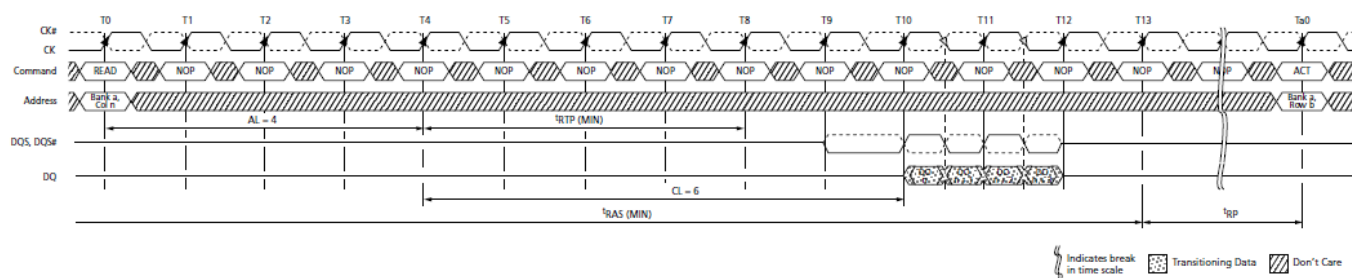
READ with Auto Precharge (AL = 4, CL = 6)
